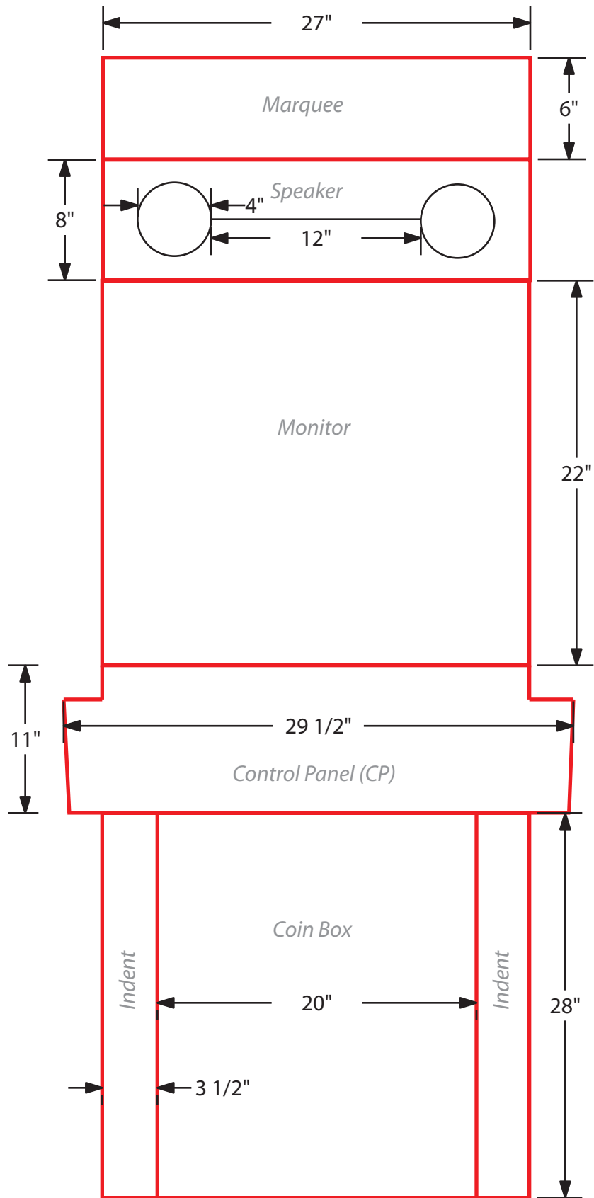
Cabinet Front
